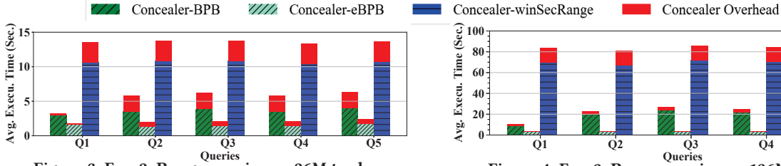
Figure 3: Exp 2: Range queries on 26M tuples.
