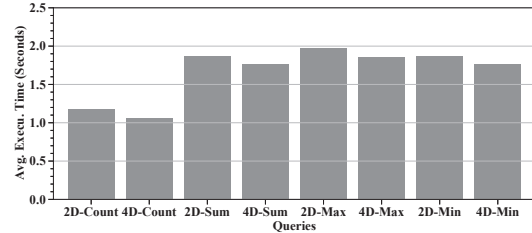
Figure 6: Exp 5: Query performance on TPC-H data.
